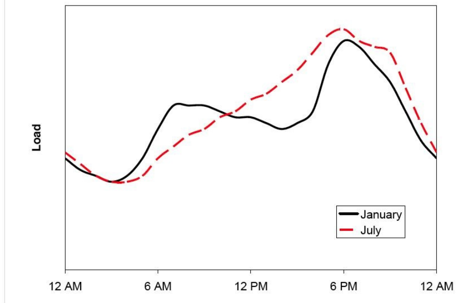
Figure 7. A typical 24 hour load profile for a residence in San Jose, CA. (Source: NREL)
