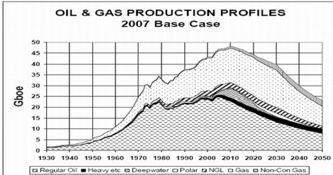
Fig.8: Peak oil and gas – source: C. Campbell, ASPO Ireland
