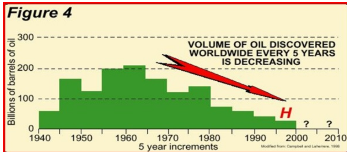
Fig.10: New oil discoveries – source: L. Magoon, U.S. Geological Survey
