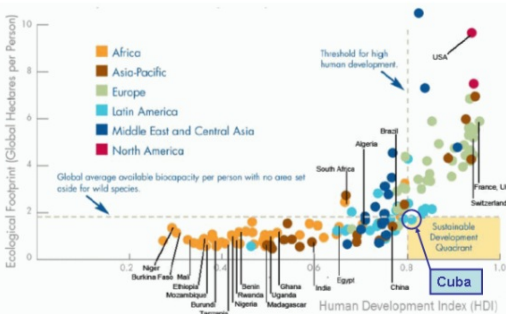
Fig.4: Ecological footprint – source: Living Planet Report 2006
