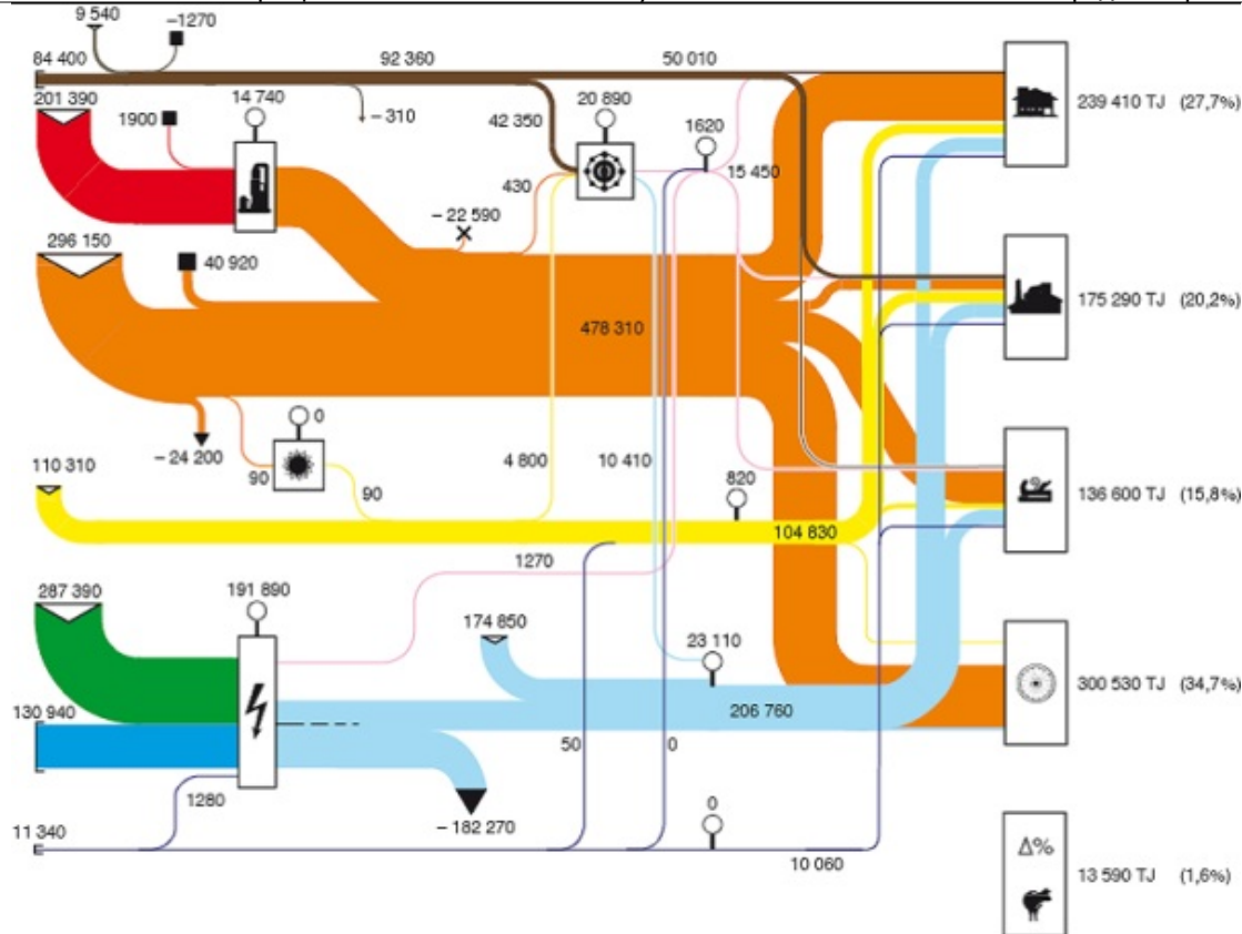
Fig.1: Sankey diagram of Switzerland - source: Dr. Michael Piot, Swiss Federal Office of Energy
