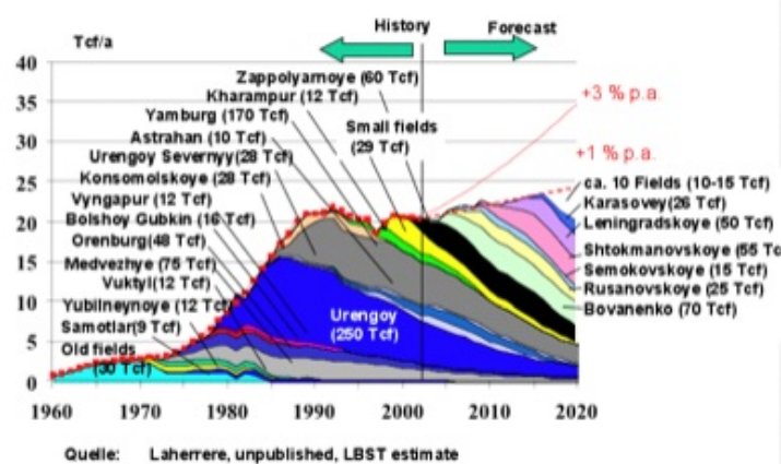
Figure 21 Russian gas production forecast by Jean Laherrere showing how second tier fields may compensate for decline in the three giants - Yamburg, Urengoy and Medvezhye.
