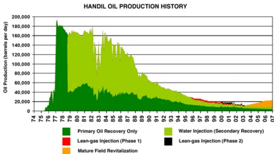
Figure 2: Handil Oil Production History
