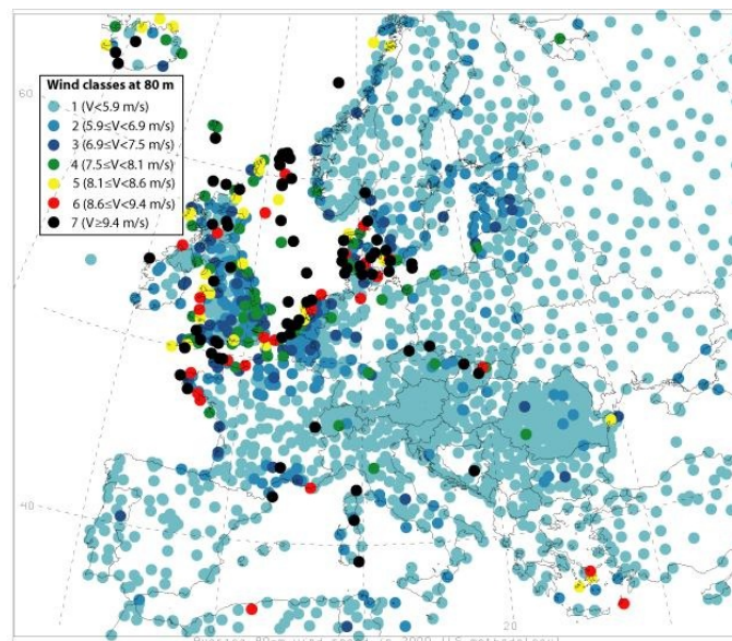
Figure 9. The distribution of wind speeds at 80 meters, the hub height of a modern turbine. (Source: Cristina L. Archer and Mark Z. Jacobson, Evaluation of global wind power) Click to Enlarge
