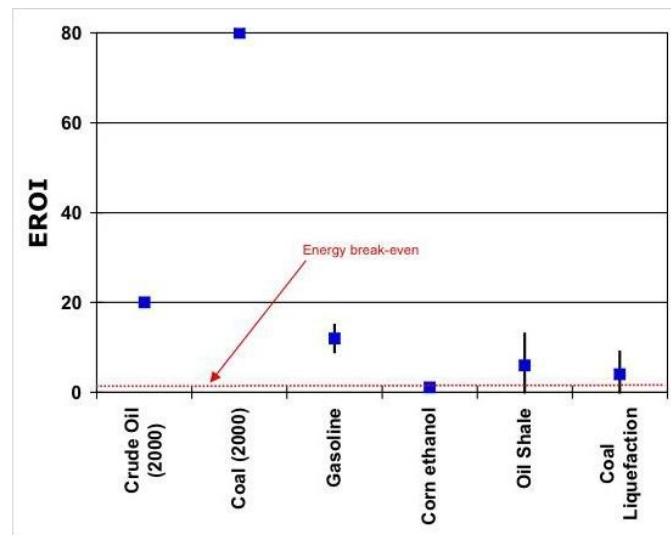
Figure 6. The energy return on investment (EROI) for various fuel sources in the U.S. (Source: Cutler Cleveland) Click to Enlarge
