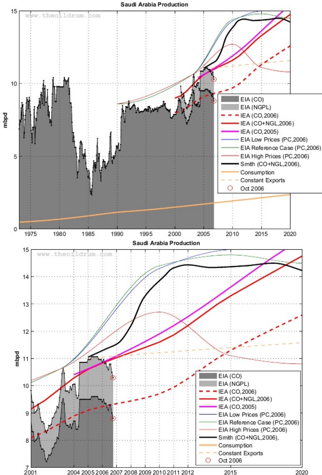
Fig 9.- Saudi Arabia oil production (EIA Monthly) and various forecasts (2001-2020). The EIA estimate is a productive capacity (PC). Click to Enlarge .
